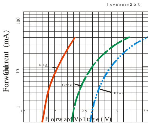
Volt-Ampere Characteristics
