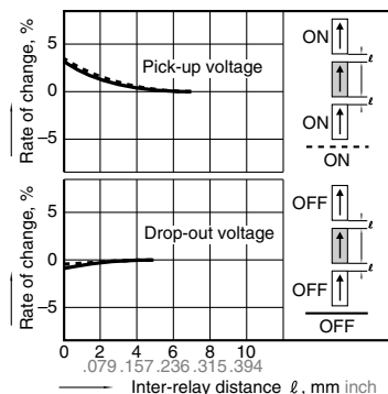
10-(2). Influence of adjacent mounting Tested sample: TX2-12V, 6 pcs.
