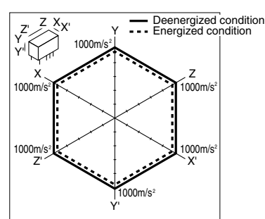
9. Malfunctional shock (single side stable) Tested sample: TX2-5V, 6 pcs.
