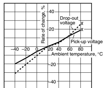
7. Ambient temperature characteristics Tested sample: TX2-5V, 5 pcs.
