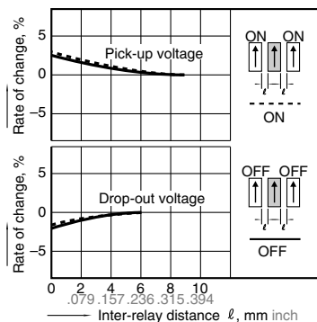
10-(1). Influence of adjacent mounting Tested sample: TX2-12V, 6 pcs.
