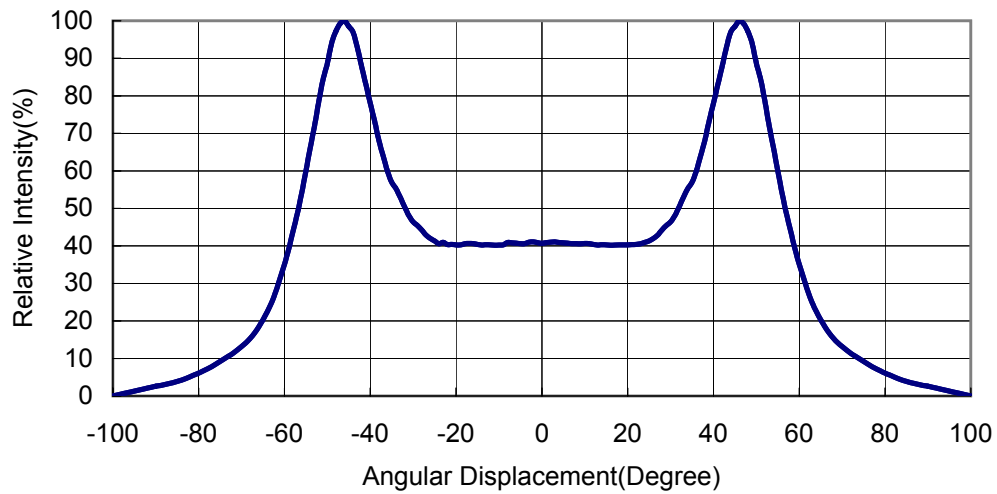
Fig 6. Typical Representative Spatial Radiation Pattern for White, Warm White, Blue, Green, Amber, Red-Orange and Red.
