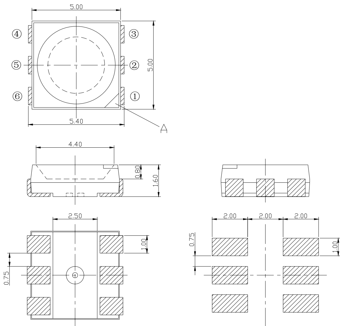
推荐焊盘 Recommended Soldering Pad
