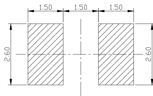
Recommned Soldering Pad
