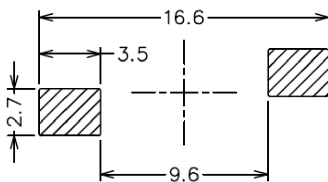
Soldering patterns
