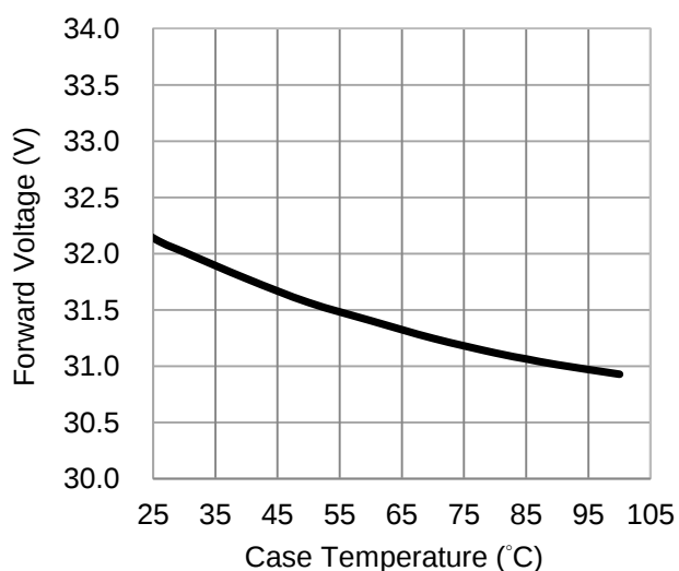
Fig 2. Case Temperature vs. Forward Voltage at 3100mA.
