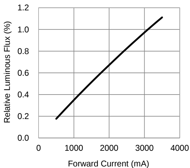
Fig 6. Forward Current vs. Relative Luminous Flux at T_C=25^{\circ}\text{C} .
