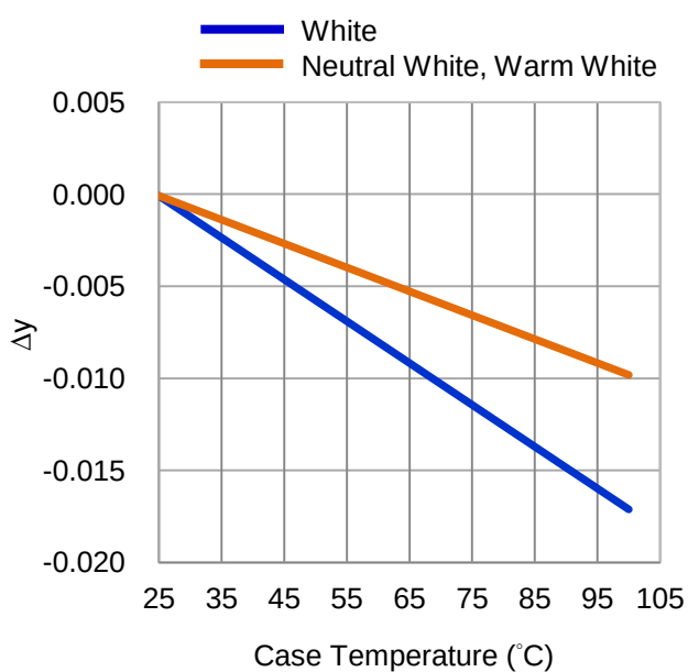
Fig 4. Case Temperature vs. Chromaticity Coordinate \Delta y at 480mA.
