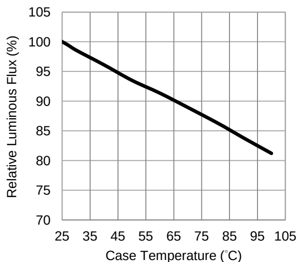
Fig 1. Case Temperature vs. Relative Luminous Flux at 480mA.
