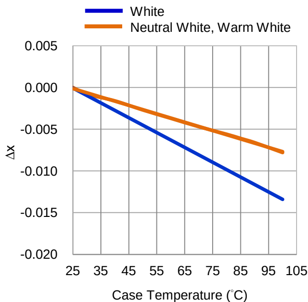
Fig 3. Case Temperature vs. Chromaticity Coordinate \Delta x at 480mA.
