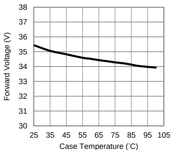
Fig 2. Case Temperature vs. Forward Voltage at 480mA.
