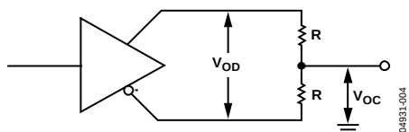
Figure 18. Driver Voltage Measurement
