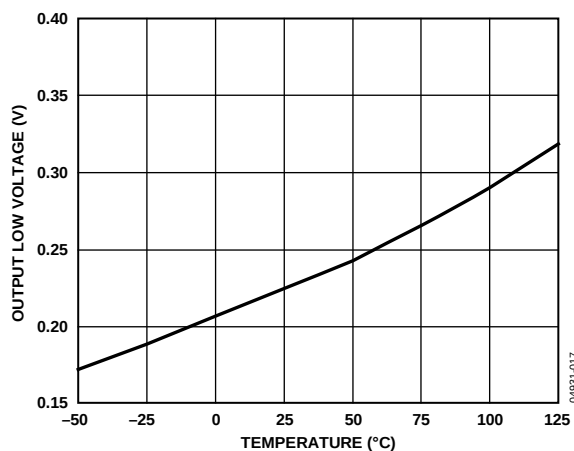
Figure 9. Receiver Output Low Voltage vs. Temperature
