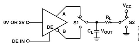
Figure 21. Driver Enable/Disable (ADM4850/ADM4852/ADM4853)
