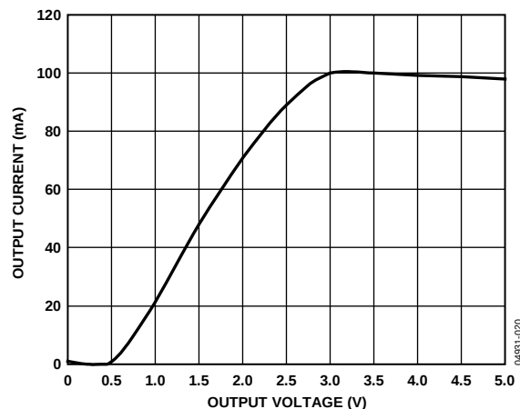
Figure 12. Output Current vs. Driver Output Low Voltage
