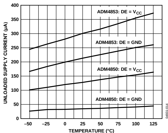
Figure 6. Unloaded Supply Current vs. Temperature (ADM4850/ADM4853)
