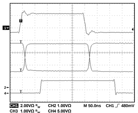
Figure 17. Driver/Receiver Propagation Delay (ADM4857, 4 Mbps)
