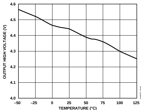
Figure 10. Receiver Output High Voltage vs. Temperature
