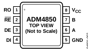
Figure 3. 8-Lead MSOP Pin Configuration, ADM4850
