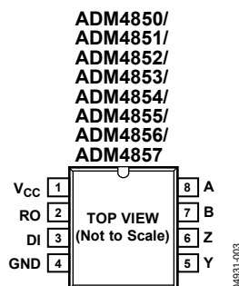
Figure 5. 8-Lead SOIC Pin Configuration, ADM4850/ADM4851/ADM4852/ADM4853/ADM4854/ADM4855/ADM4856/ADM4857
