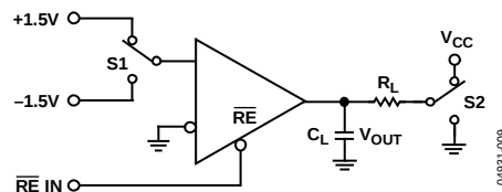
Figure 23. Receiver Enable/Disable (ADM4850/ADM4852/ADM4853)
