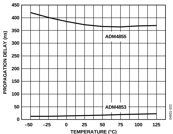
Figure 14. Driver Propagation Delay vs. Temperature (ADM4853/ADM4855)
