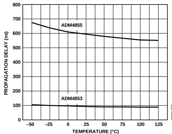
Figure 15. Receiver Propagation Delay vs. Temperature (ADM4853/ADM4855)
