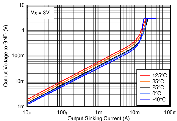
Figure 6-22. Output Low Voltage vs. Output Sinking Current at 3V
