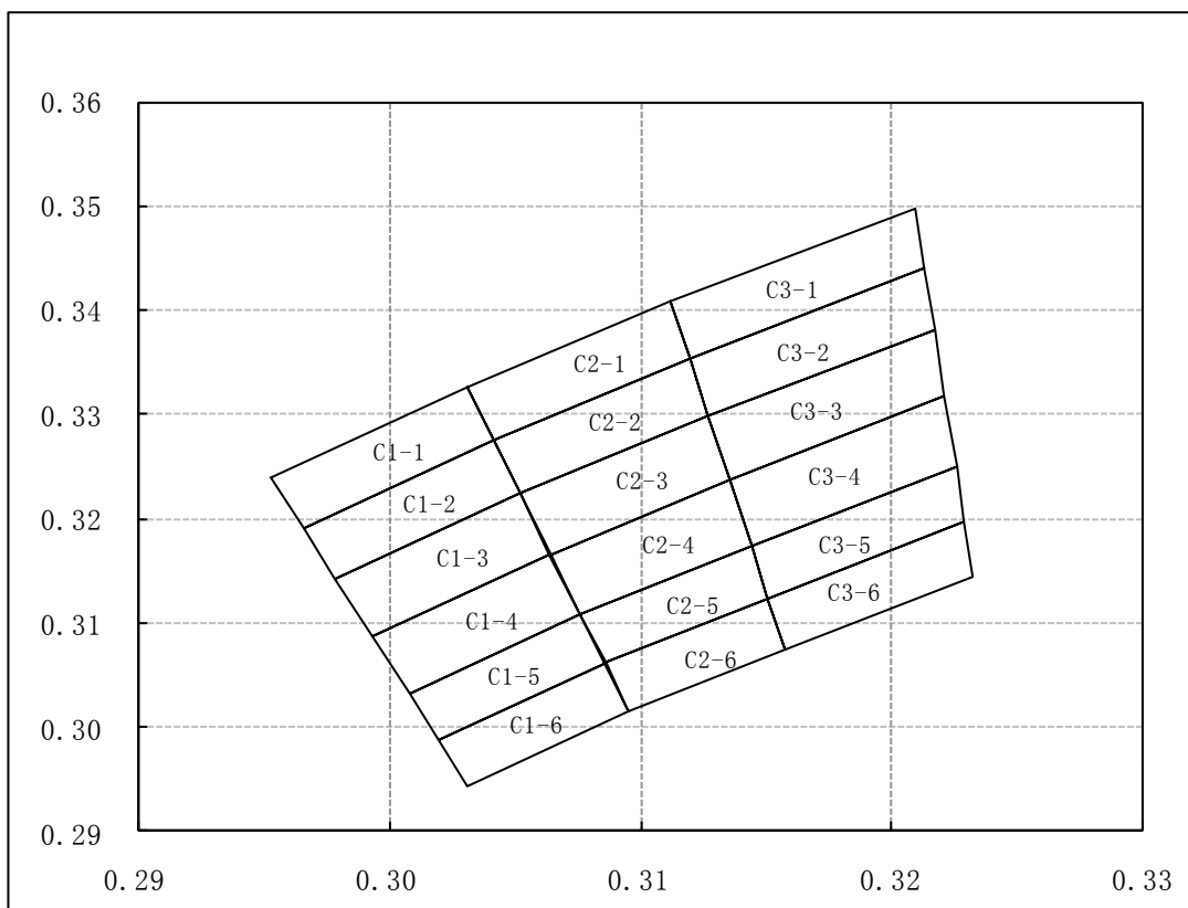
CIE Chromaticity Diagram
