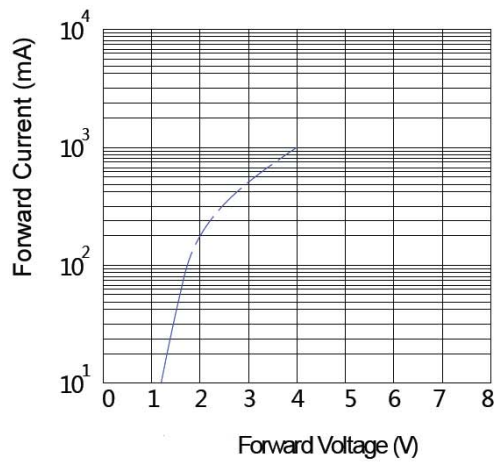
Current & Voltage Curve
