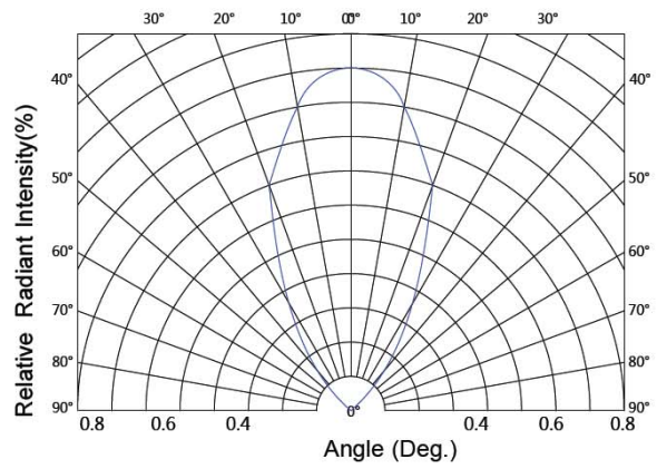
Radiant Intensity Spatial Distribution
