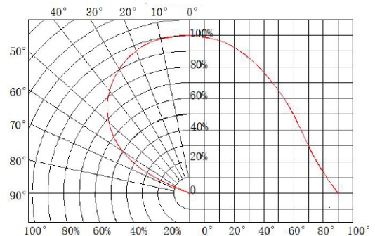
Radiation diagram
