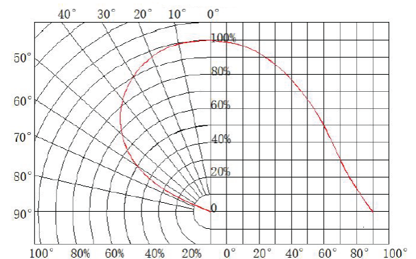
Radiation diagram
