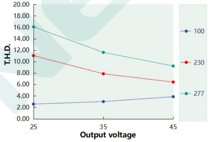
T.H.D. VS Output voltage ( DL-60Z-AC1350-MAC )
