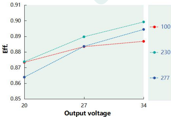
Eff. VS Output voltage ( DL-60Z-AC1800-MAC )
