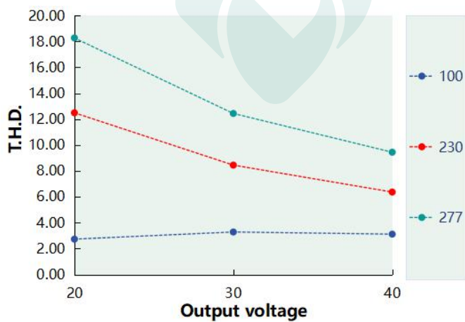
T.H.D. VS Output voltage ( DL-60Z-AC1500-MAC )
