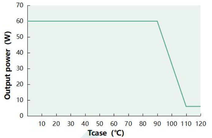
Output power VS Tcase(DL-60Z-AC-MAC )
