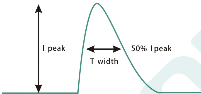
Inrush Current ( DL-60Z-AC-MAC )
