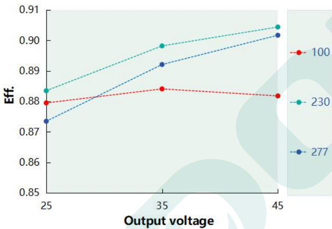
Eff. VS Output voltage ( DL-60Z-AC1350-MAC )
