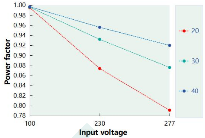
Power Factor VS Input Voltage ( DL-60Z-AC1500-MAC )
