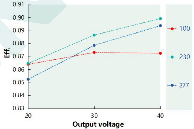
Eff. VS Output voltage ( DL-60Z-AC1500-MAC )
