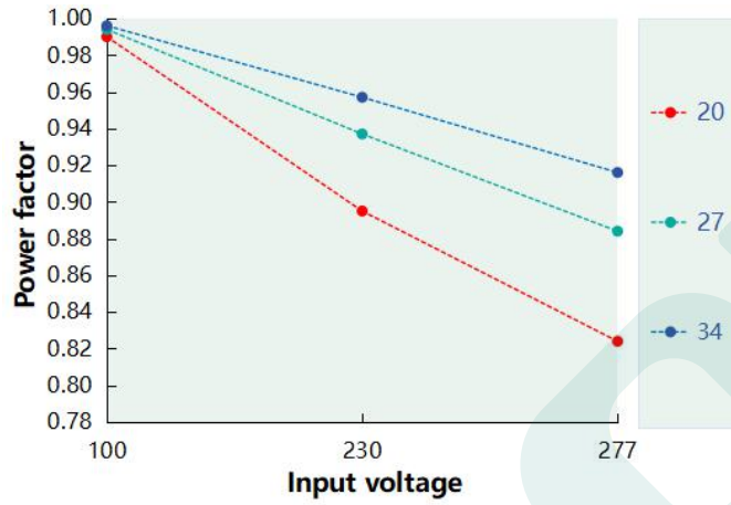
Power Factor VS Input Voltage ( DL-60Z-AC1800-MAC )
