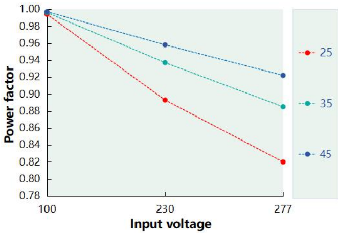
Power Factor VS Input Voltage ( DL-60Z-AC1350-MAC )
