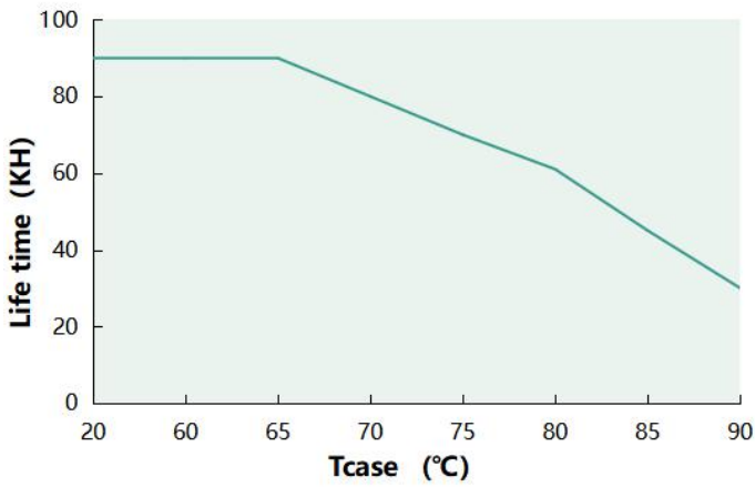
Lifetime VS Tcase ( DL-60Z-AC-MAC )
