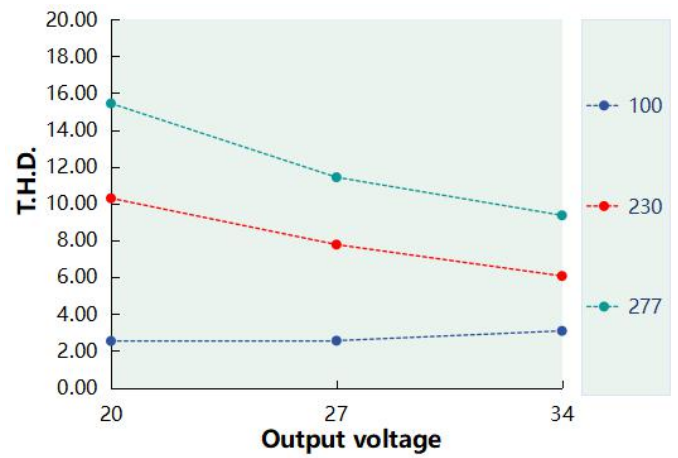
T.H.D. VS Output voltage ( DL-60Z-AC1800-MAC )
