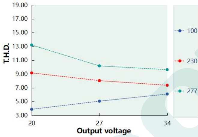
T.H.D. VS Output voltage ( DL-40Z-AC1200-MAC )
