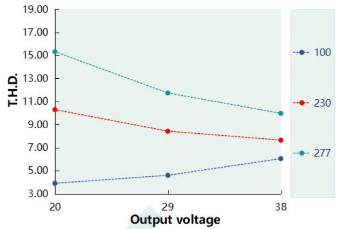
T.H.D. VS Output voltage ( DL-40Z-AC1050-MAC )
