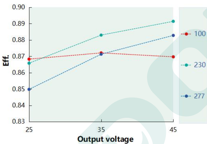
Eff. VS Output voltage ( DL-40Z-AC900-MAC )
