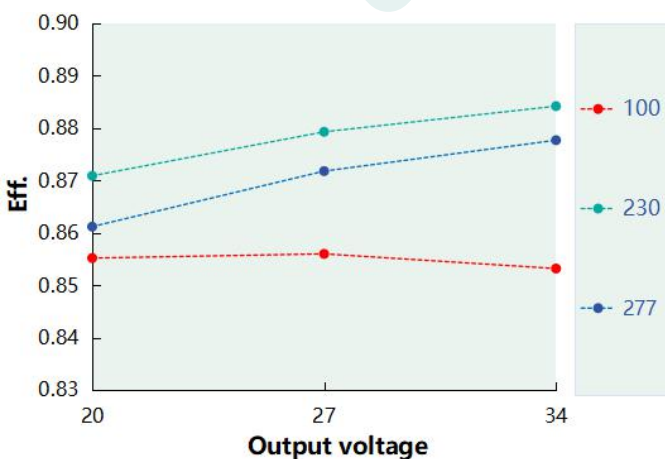
Eff. VS Output voltage ( DL-40Z-AC1200-MAC )
