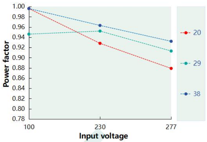
Power Factor VS Input Voltage ( DL-40Z-AC1050-MAC )
