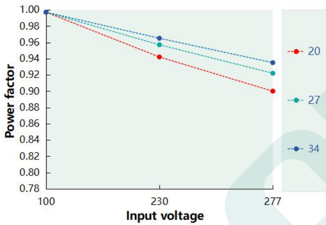
Power Factor VS Input Voltage ( DL-40Z-AC1200-MAC )
