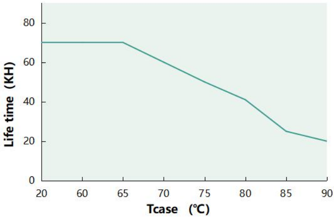
Lifetime VS Tcase ( DL-40Z-AC-MAC )
