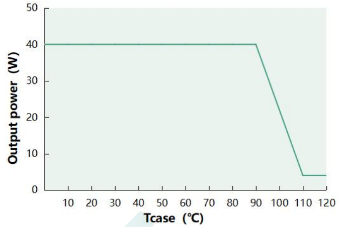
Output power VS Tcase ( DL-40Z-AC-MAC )
