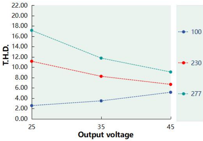
T.H.D. VS Output voltage ( DL-40Z-AC900-MAC )
