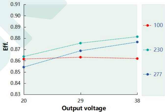
Eff. VS Output voltage ( DL-40Z-AC1050-MAC )
