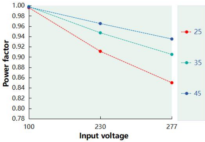
Power Factor VS Input Voltage ( DL-40Z-AC900-MAC )
