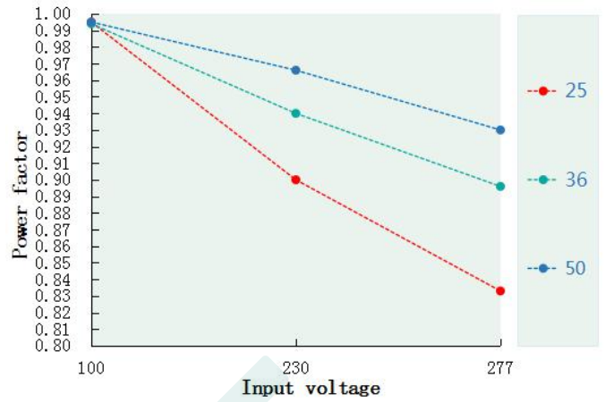
Power factor VS Input voltage(DL-50Z-C1050-MAC )
