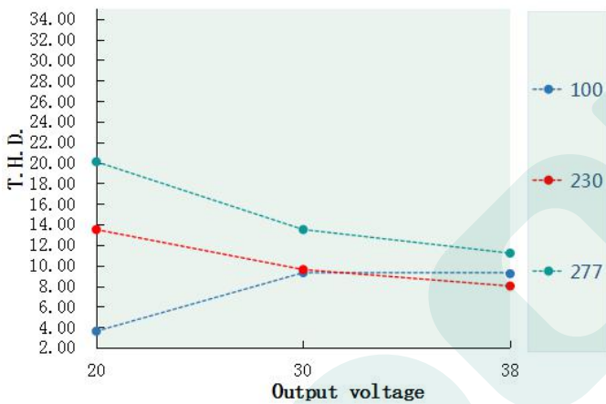
T.H.D. VS Output voltage(DL-50Z-C1200-MAC )
