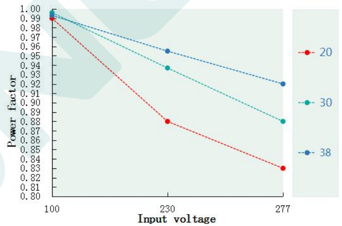
Power factor VS Input voltage(DL-50Z-C1350-MAC )
