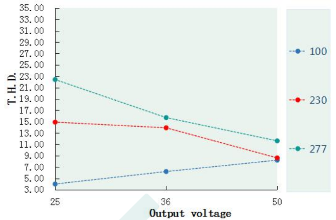
T.H.D. VS Output voltage(DL-50Z-C1050-MAC )
