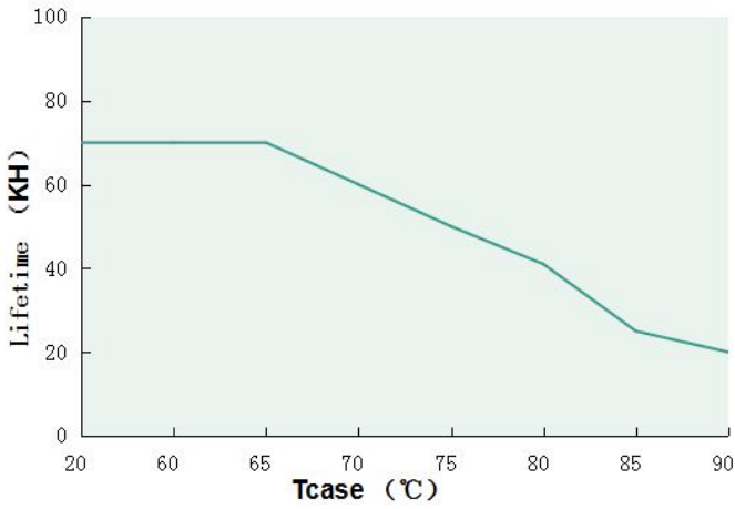
Tcase VS Lifetime (DL-50Z-MAC)
