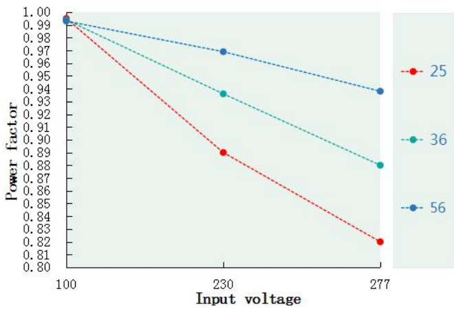
Power factor VS Input voltage(DL-50Z-C900-MAC )
