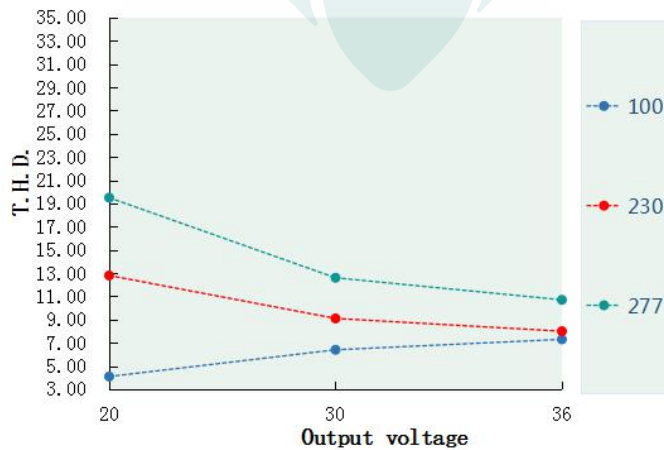
T.H.D. VS Output voltage(DL-50Z-C1500-MAC )
