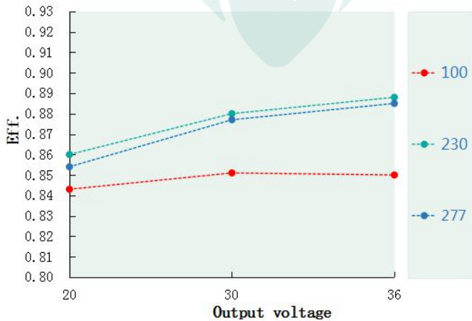
Eff. VS Output voltage(DL-50Z-C1500-MAC )
