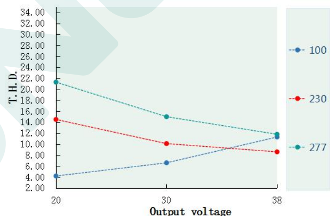
T.H.D. VS Output voltage(DL-50Z-C1350-MAC )
