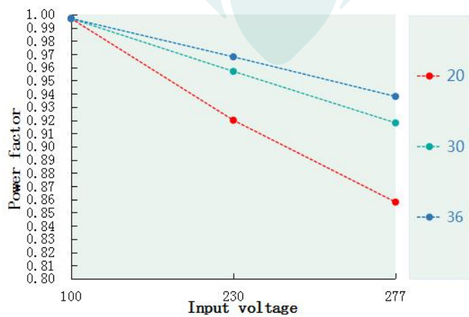
Power factor VS Input voltage(DL-50Z-C1500-MAC )
