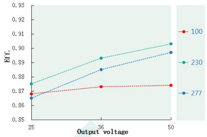
Eff. VS Output voltage(DL-50Z-C1050-MAC )
