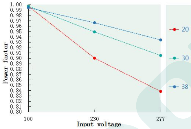
Power factor VS Input voltage(DL-50Z-C1200-MAC )
