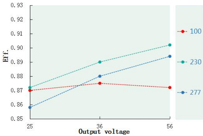
Eff. VS Output voltage(DL-50Z-C900-MAC )
