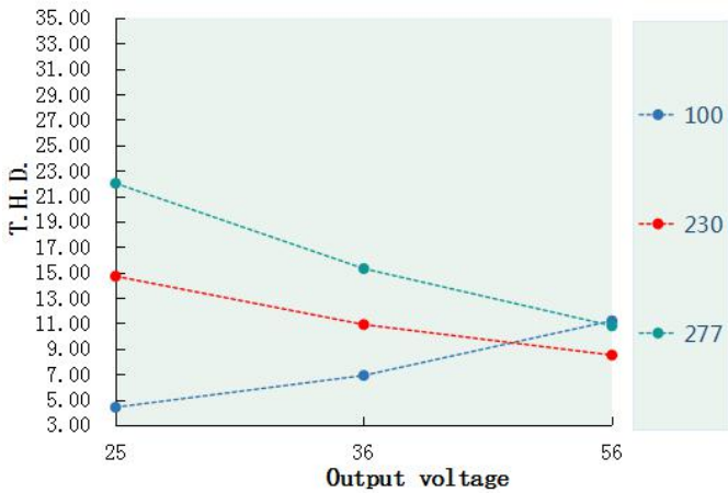
T.H.D. VS Output voltage(DL-50Z-C900-MAC )
