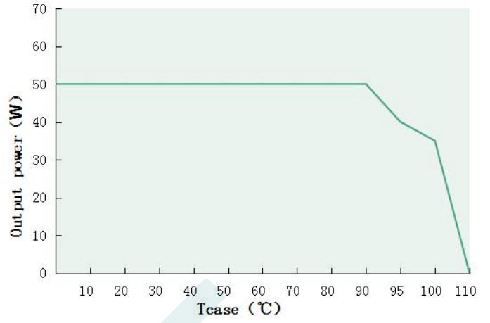
Output power VS Tcase (DL-50Z-MAC)
