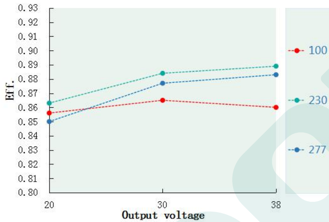
Eff. VS Output voltage(DL-50Z-C1200-MAC )
