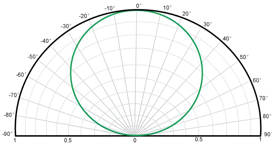
Fig.3 Typical radiation pattern in polar coordinate system
