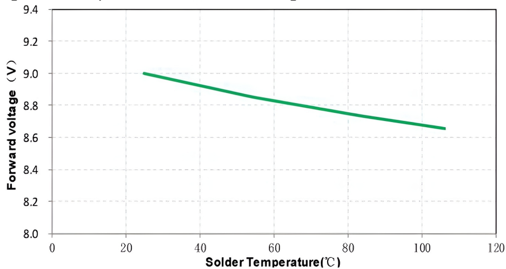
Fig.1 Pad temperature and forward voltage characteristic curve
