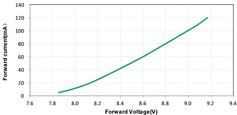
Fig.2 Forward voltage and forward current characteristic curves
