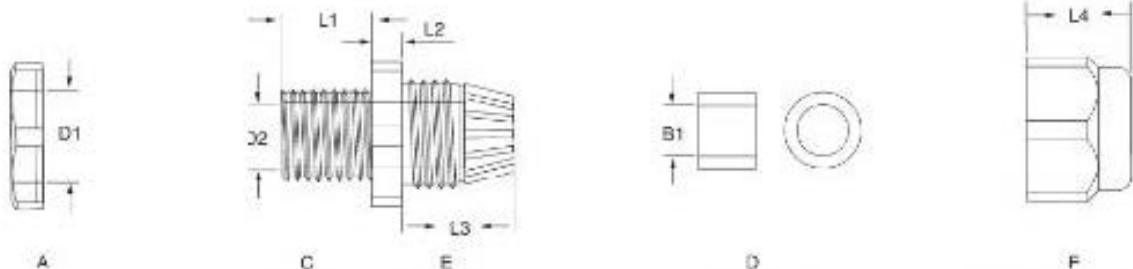
A 螺帽 Lock nut
