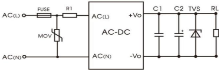
Fig. 2: EMC application circuit with higher requirements
