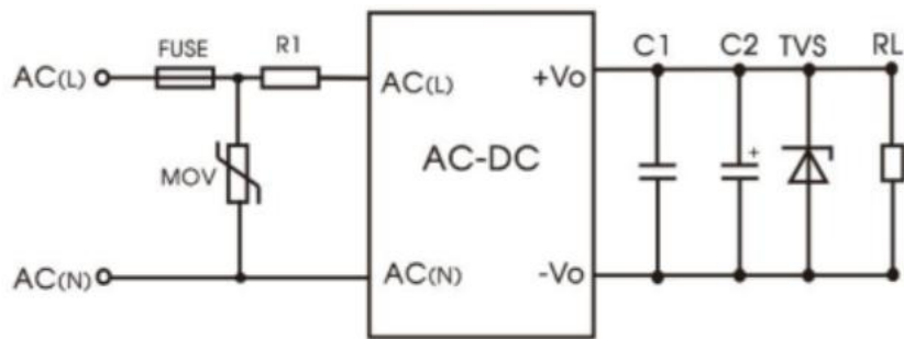
Fig. 1: Typical circuit diagram
