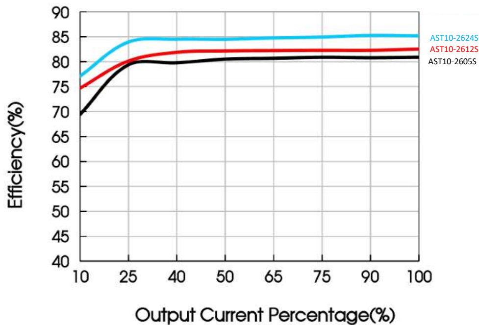
Efficiency Vs Output Load (Vin=230VAC)
