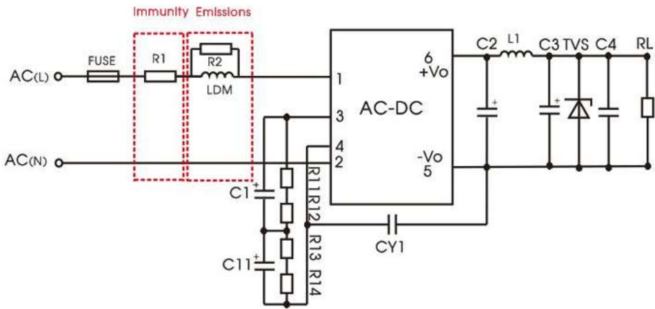
Recommended circuit 1
