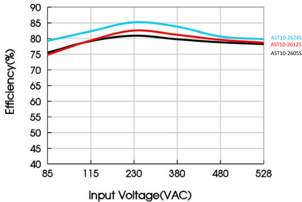
Efficiency Vs Input Voltage (Full Load)
