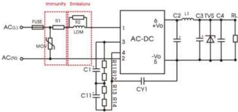
Recommended circuit 4
