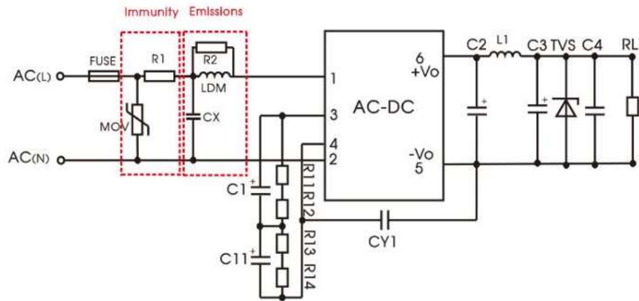
Recommended circuit 3
