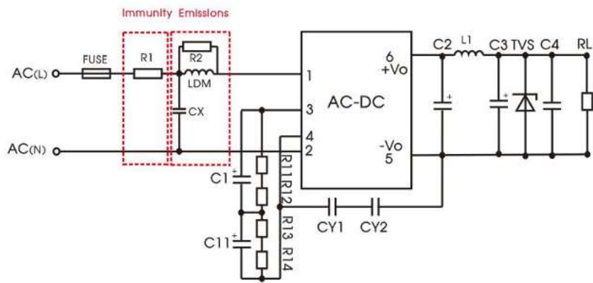
Recommended circuit 2
