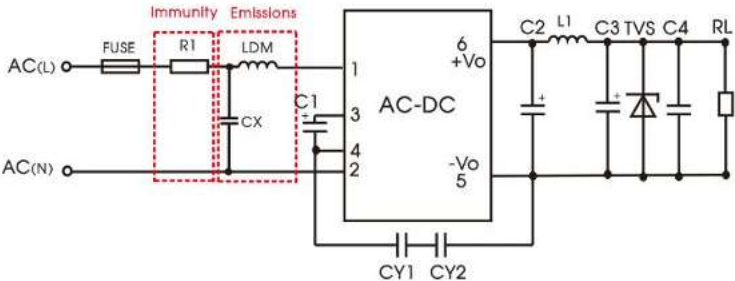
Recommended circuit 2
