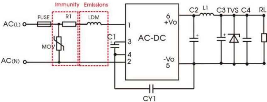
Recommended circuit 4
