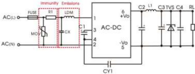
Recommended circuit 3
