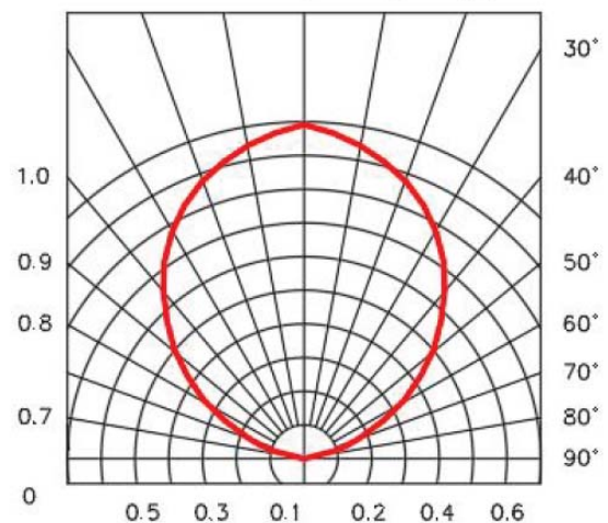
Radiation diagram 0° 10° 20°
