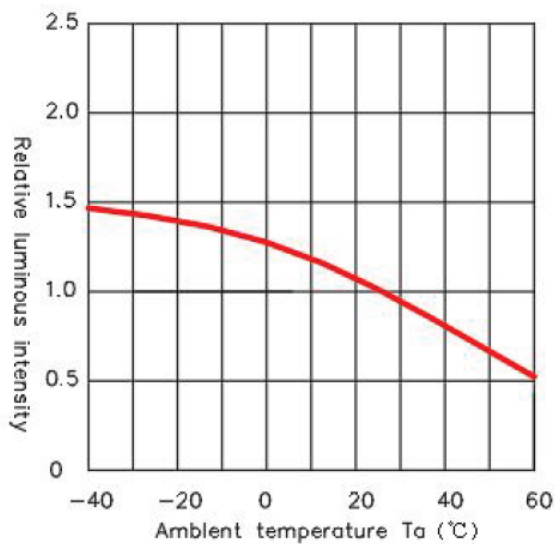
Ambient temperature Vs. Relative luminous intensity
