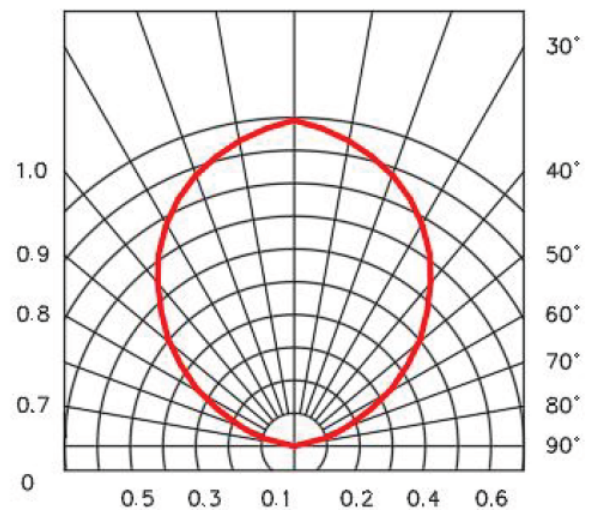
Radiation diagram 0° 10° 20°
