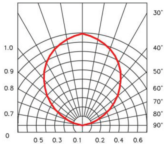
Radiation diagram 0° 10° 20°
