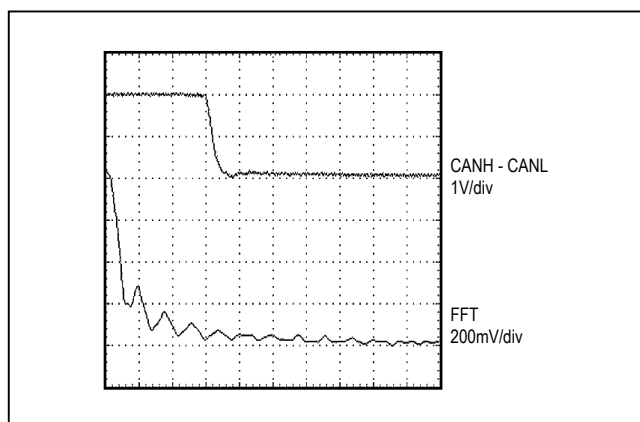
Figure 6. FFT Recessive Bus at 2Mbps
