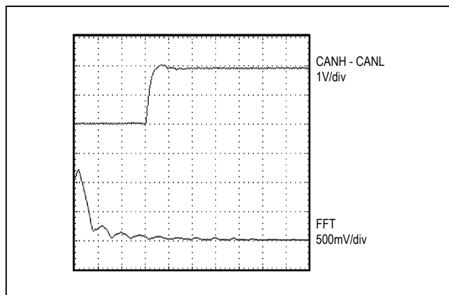
Figure 5. FFT Dominant Bus at 2Mbps layout.
