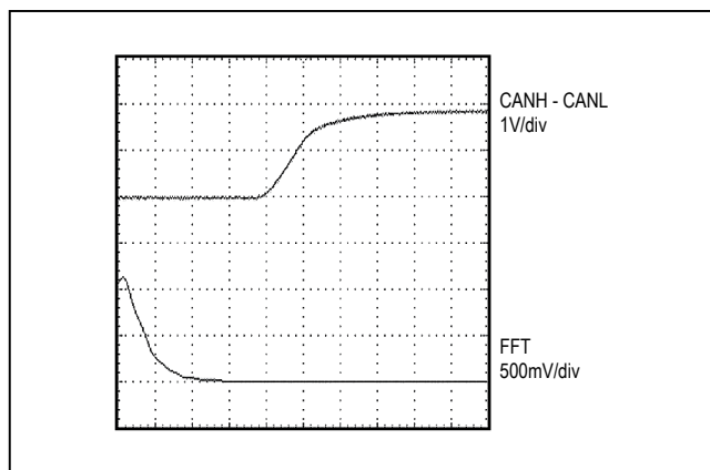
Figure 7. FFT Dominant Bus at 500kbps
