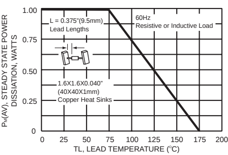
FIG. 5 - STEADY STATE POWER DERTING CURVE
