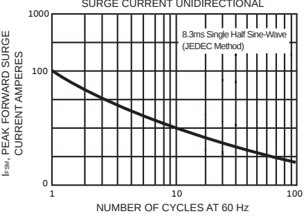
FIG. 6 - MAXIMUM NON-REPETITIVE FORWARD SURGE CURRENT UNIDIRECTIONAL
