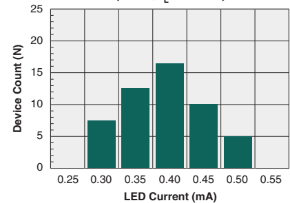
Typical I_F for Switch Dropout (N=50, I_L=100\text{mA} )
