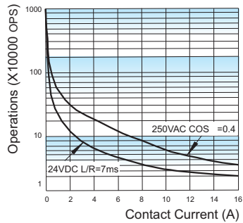
ENDURANCE CURVE(Inductive)
