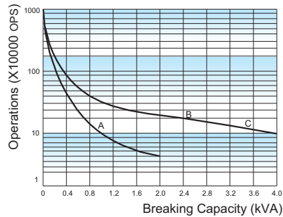
ENDURANCE CURVE(Resistive)
