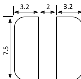
PCB PATTERN
