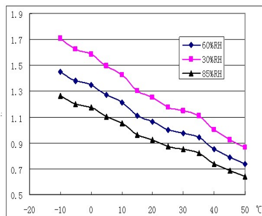
Fig4. Typical temperature/humidity characteristics
