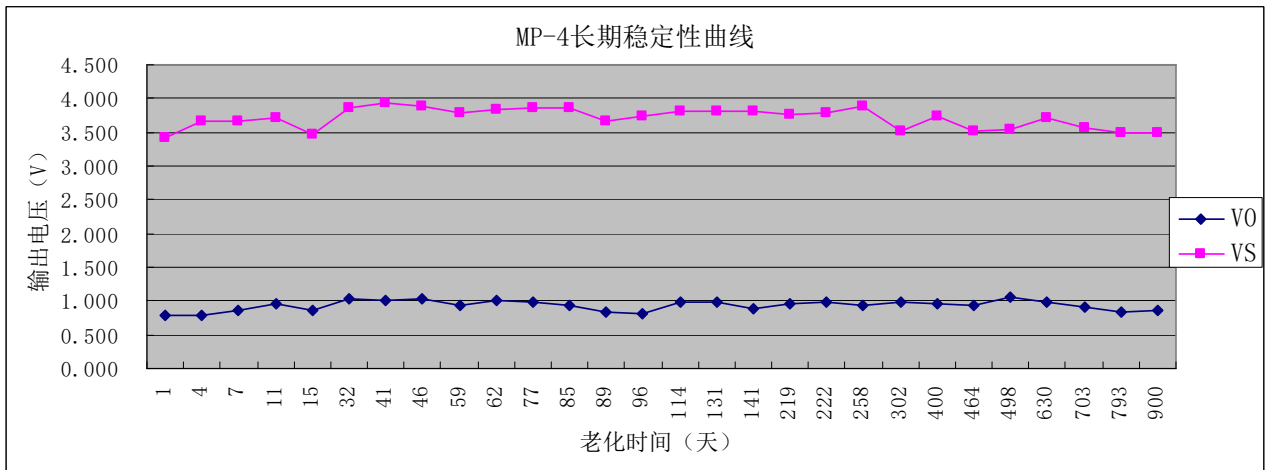
Fig7. Long-term Stability
