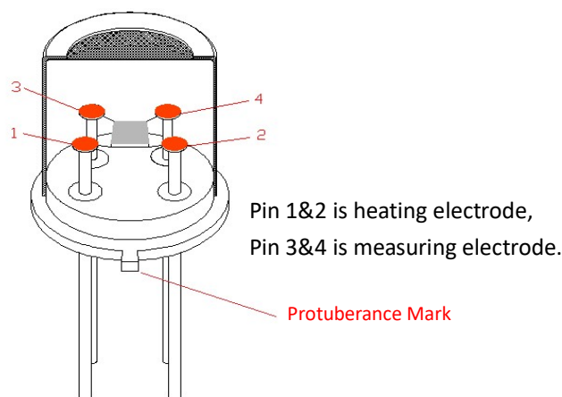
Fig8.Pin Schematic Diagram
