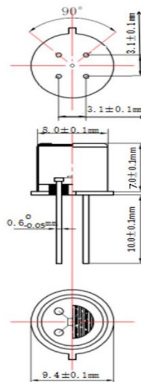
Fig1. Sensor structure
