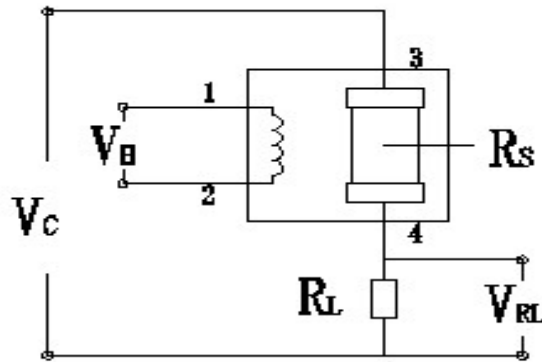
Fig2.Test circuit for MP-4
