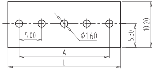
PCB LAYOUT S=1.5:1
