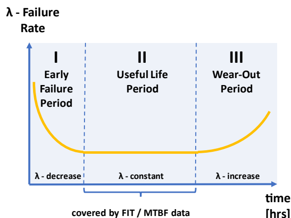
Bathtub curve
