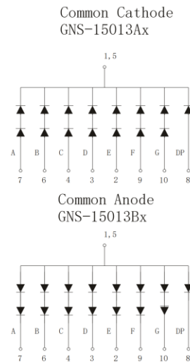
INTERNAL CIRCUIT DIAGRAM
