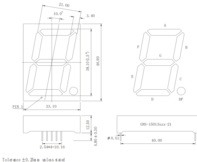
PACKAGE DIMENSION
