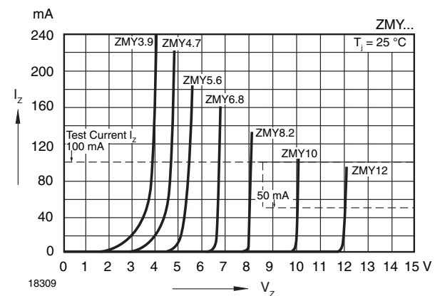
Fig. 6 - Breakdown Characteristics
