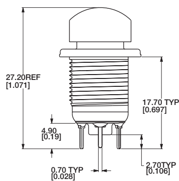
PC TERMINALS
