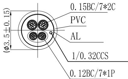
CABLE SECTION
