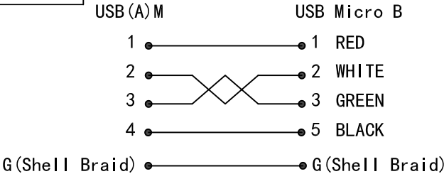
WIRING DIAGRAM
