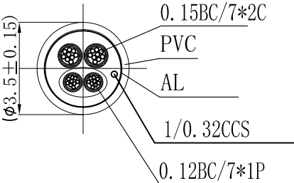
CABLE SECTION
