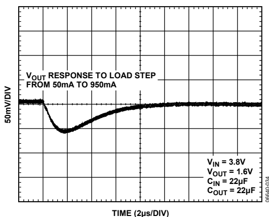
Figure 34. Output Transient Response, C_{\text{OUT}} = 22 \mu\text{F}
