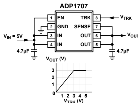
Figure 2. ADP1707 with Output Voltage Tracking
