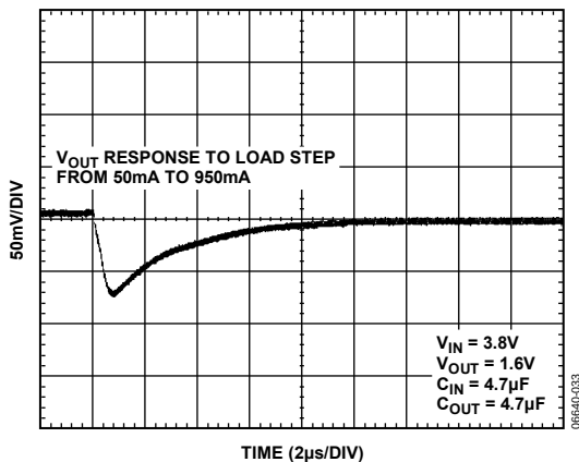
Figure 33. Output Transient Response, C_{\text{OUT}} = 4.7 \mu\text{F}
