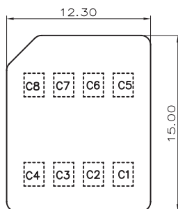
MICRO-SIM CARD DIM.(REF.)
