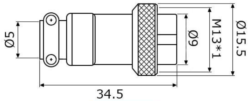
SZC-CONNECTOR
